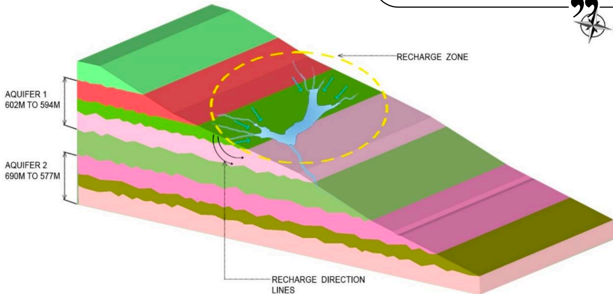
Figure 8: Combination of LS along section BB' & Geological Section showing aquifer & recharge relationships in the area
