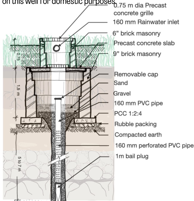
Recharge pit with perforated pipe,
