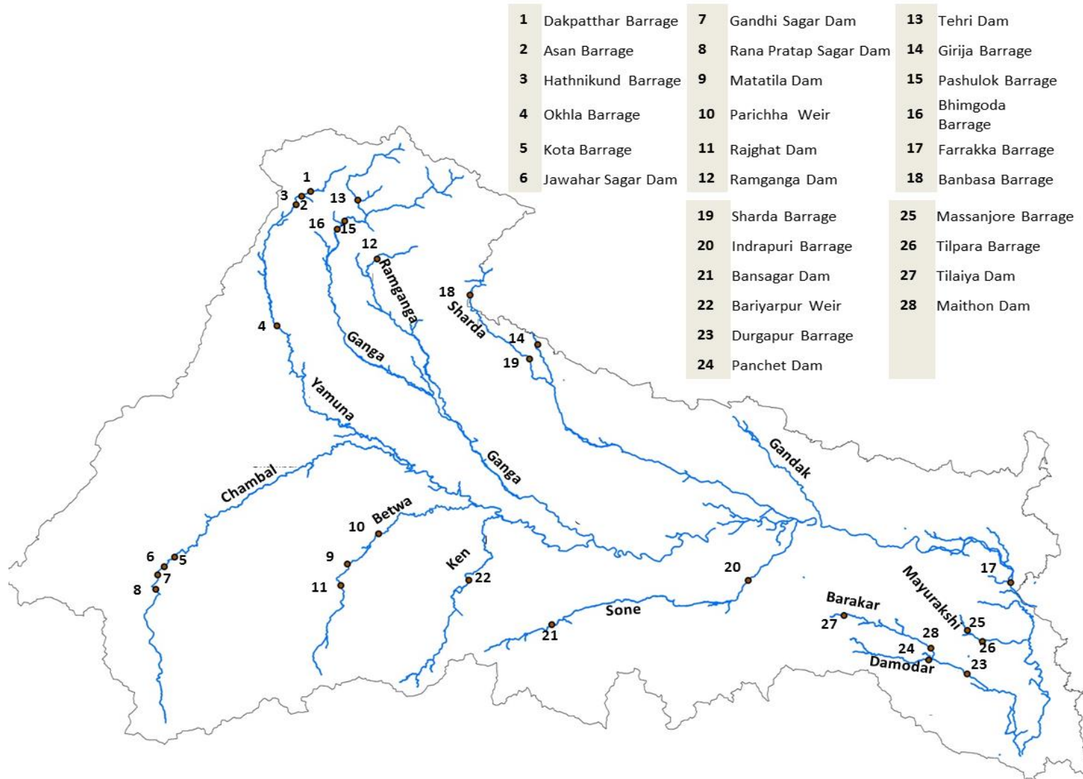
Figure 3: Major structural obstructions on River Ganga and her tributaries within India [MoWR, 2014]
