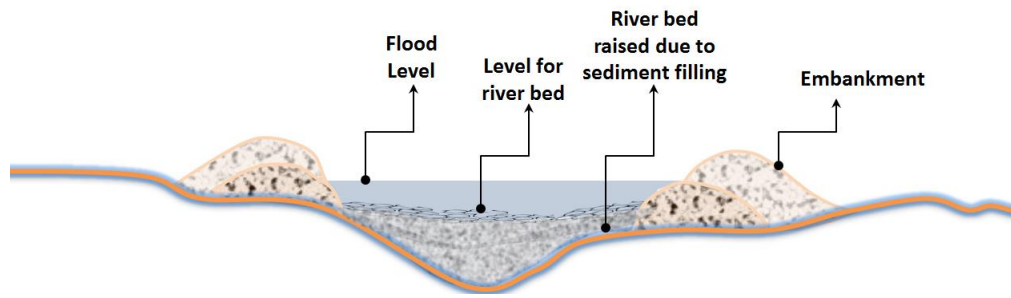
Figure 2: Cross-sectional Profile of Kosi river [adapted from Valdiya, 2011]
