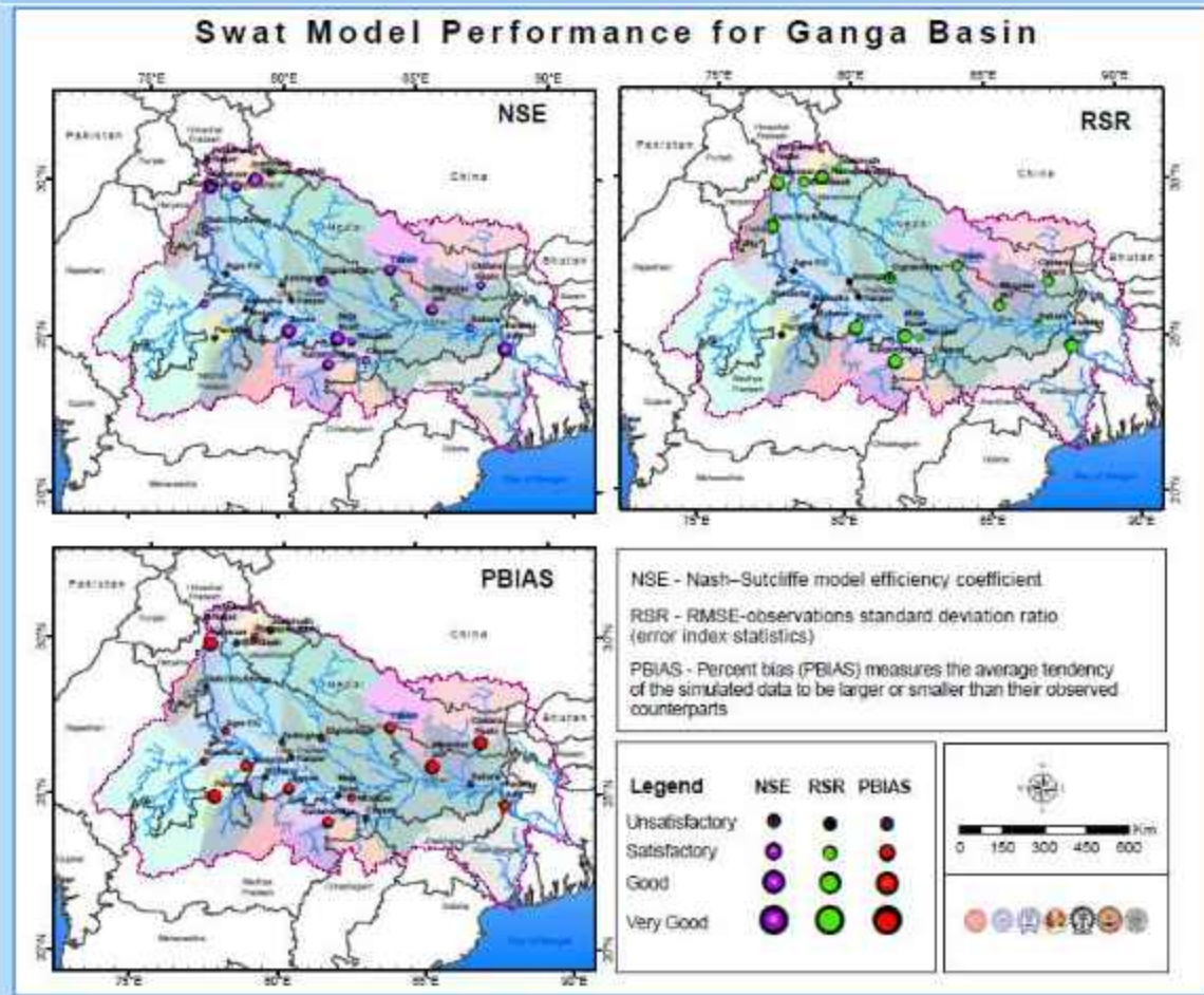
Figure 14: SWAT Model Performance for the Ganga river basin
