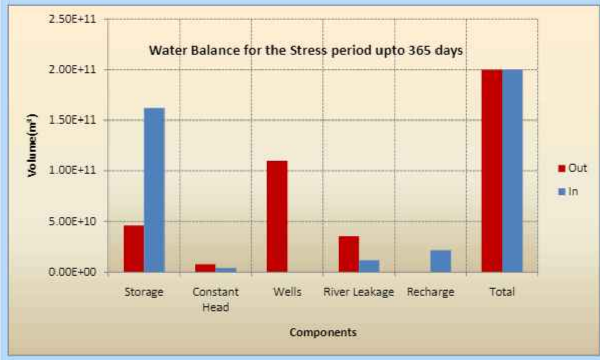
Figure 40: Mass balance for the entire study region
