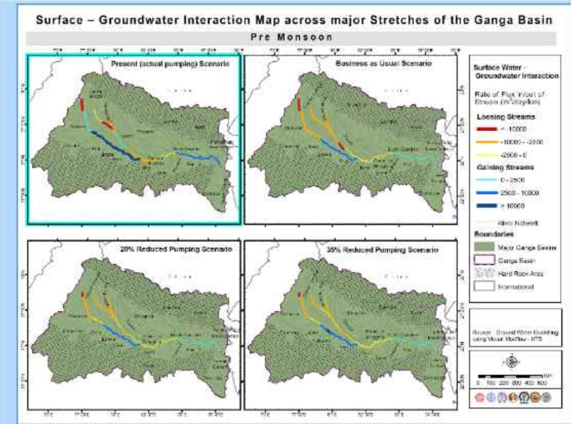
Figure 55: Plot showing the Surface GW interaction for different scenarios-Pre Monsoon
