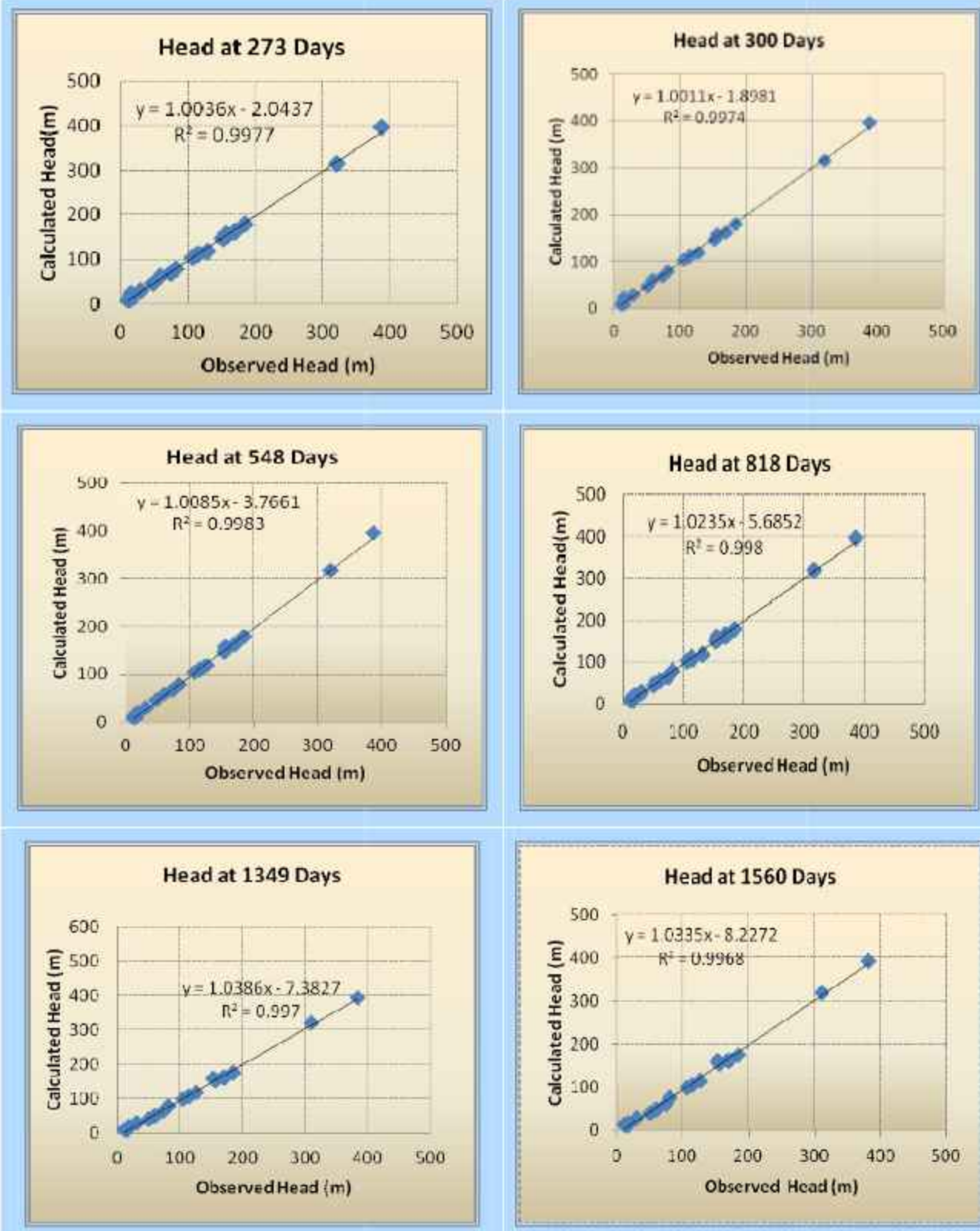
Figure 39: Scatter plot between the simulated water levels using auto calibration and observed water levels.
