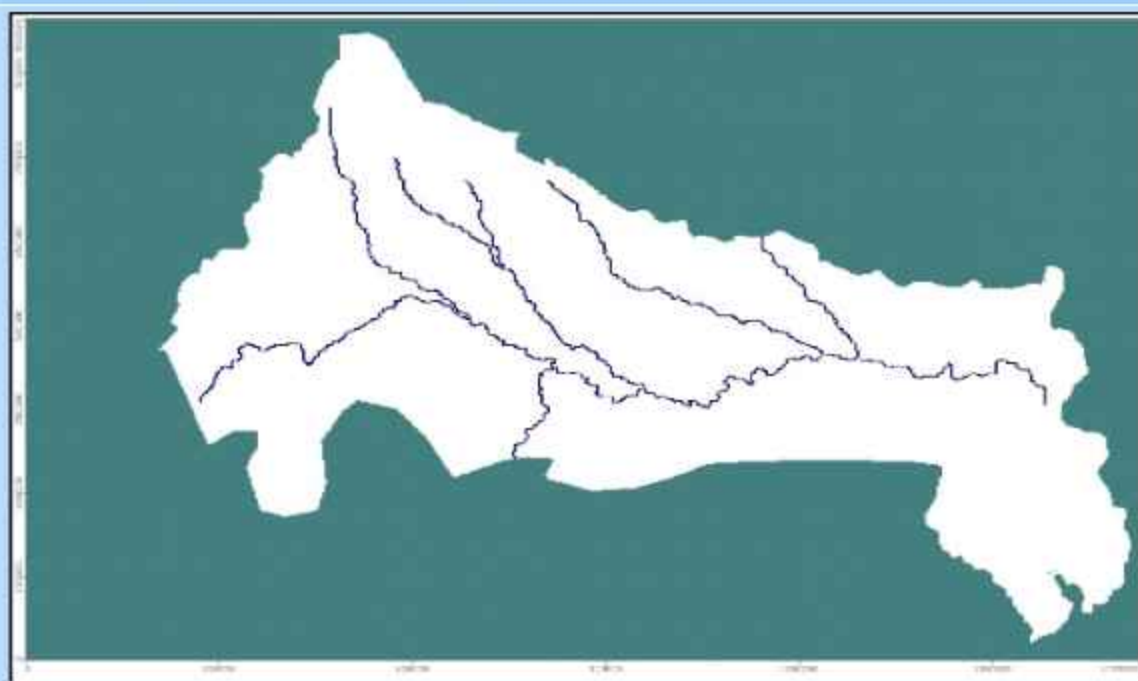
Figure 30: Incorporated River network boundary conditions in the Groundwater model
