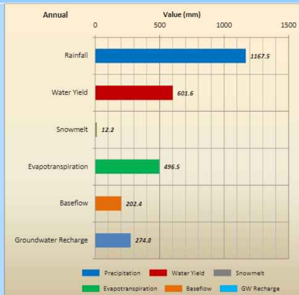
Figure 15: Annual and seasonal water balance components for the Ganga river basin
