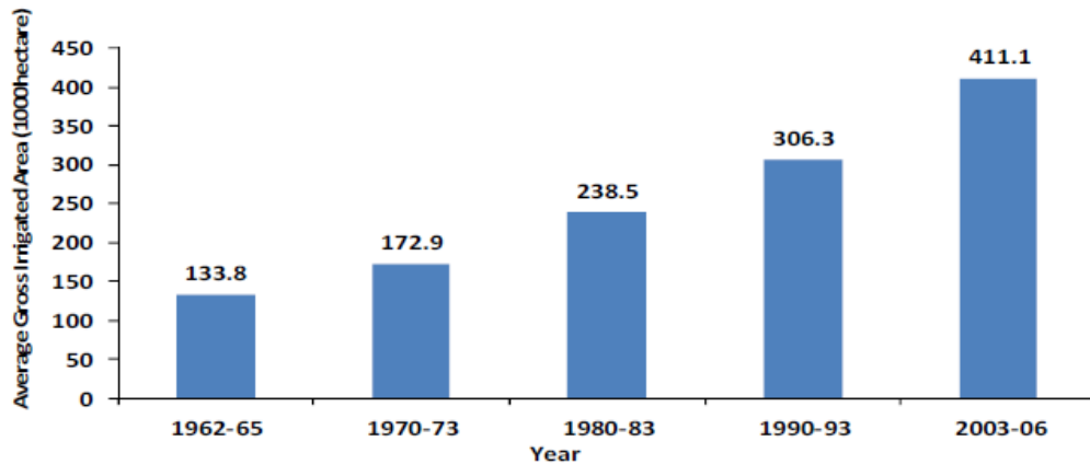
Figure 5: Average Gross Irrigated Ares (1000 hectares) per District in NRGB between 1962-65 to 2003-06 [IITC, 2011]
