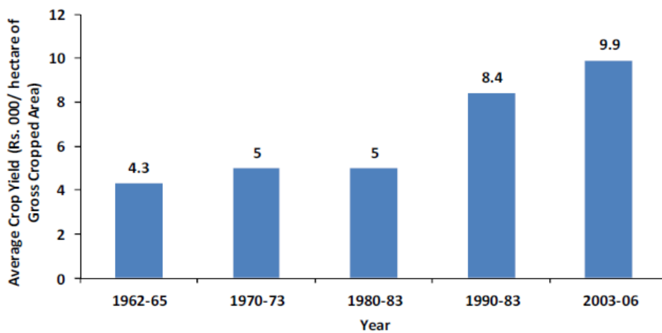
Figure 3: Average Crop Yield (Rs. 000/ hectare of Gross Cropped Area) per district in GRB, 1962-65 to 2003-06 [IITC, 2011]
