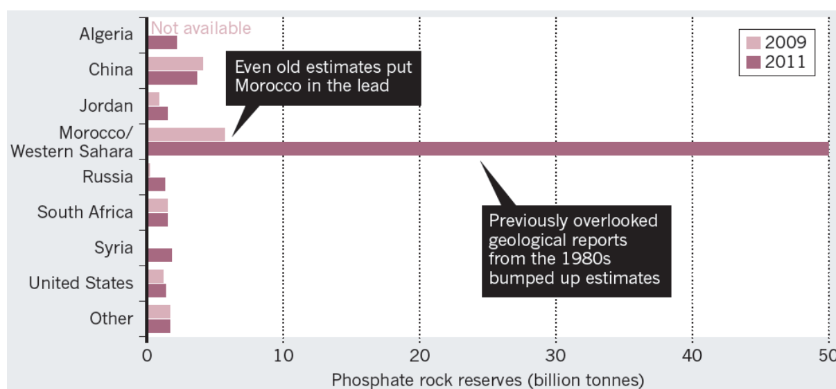
Figure 9: Global Phosphate Reserves: 2009 and 2011 estimates [Elser & Bennett, 2011]
