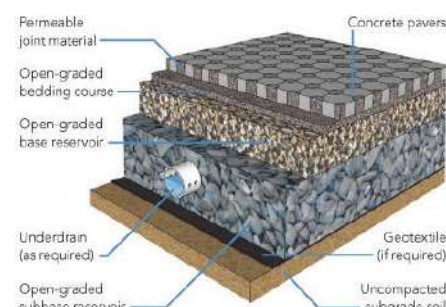
Permeable pavement
