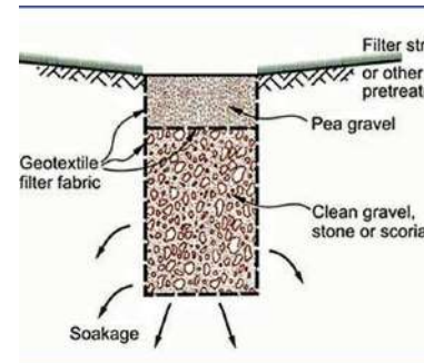
Infiltration zone
