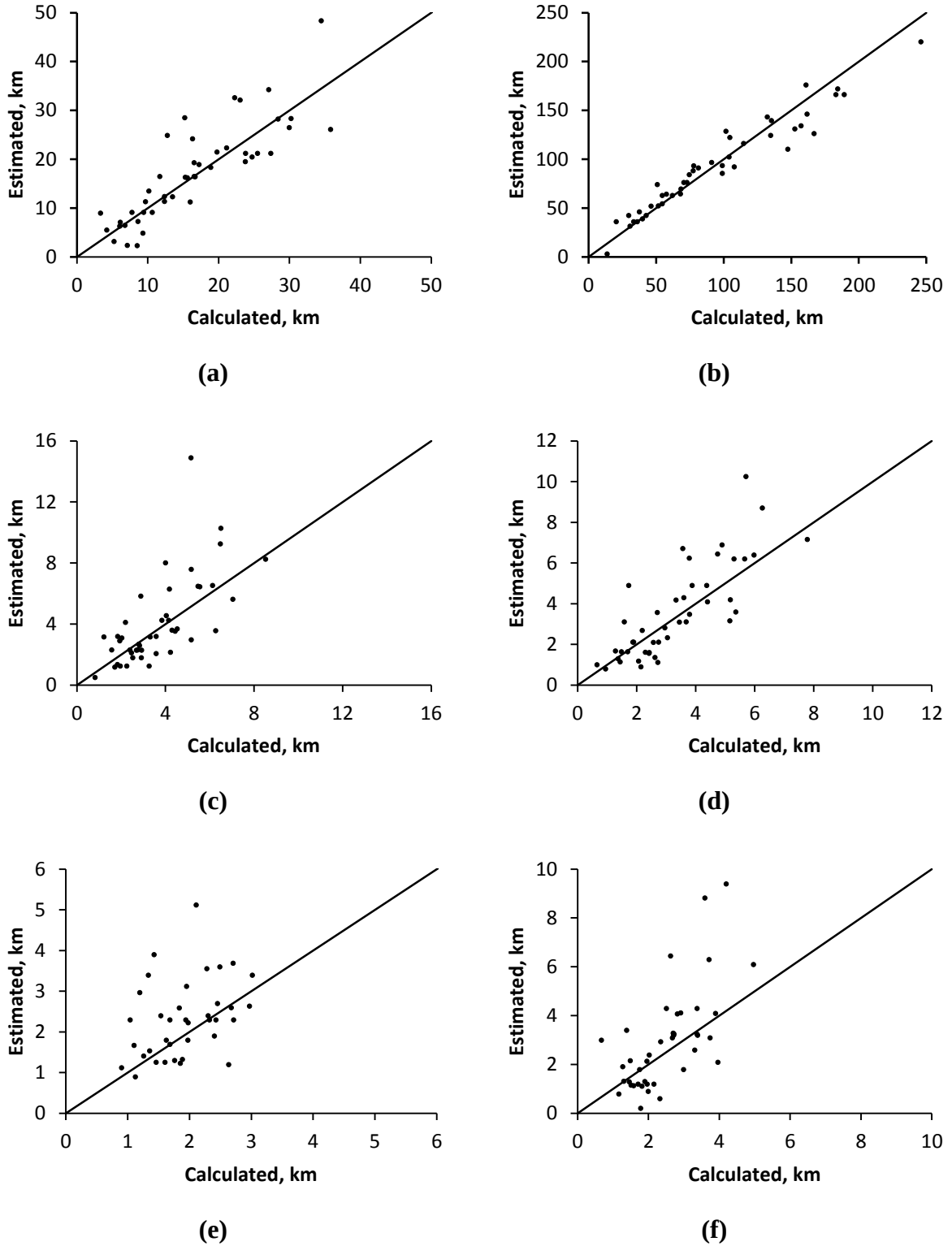
Figure 5.01: Representation of Estimated Versus Calculated Lengths of (a) 150, (b) 200, (c) 250, (d) 300, (e) 350, and (f) 400 mm Diameter Sewers
