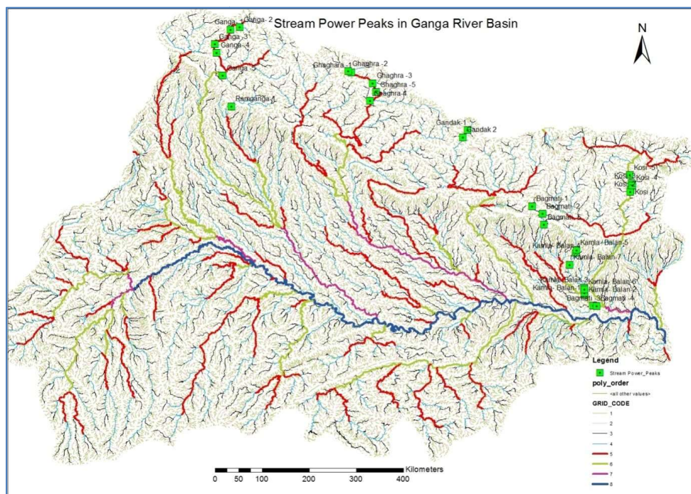
Figure 25: Location of Stream Power Peaks in the Planform Map. The Most of the Stream Power Peaks Lies it the Higher Himalayan Areas, which is also the Major Sources of Sediment Supply in Downstream Reaches.
