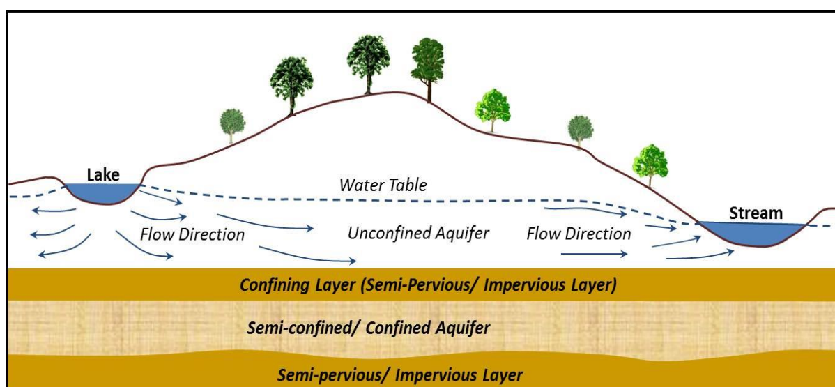
Figure 1.2: Schematic of Hydraulic Connectivity through Groundwater in NRGB
