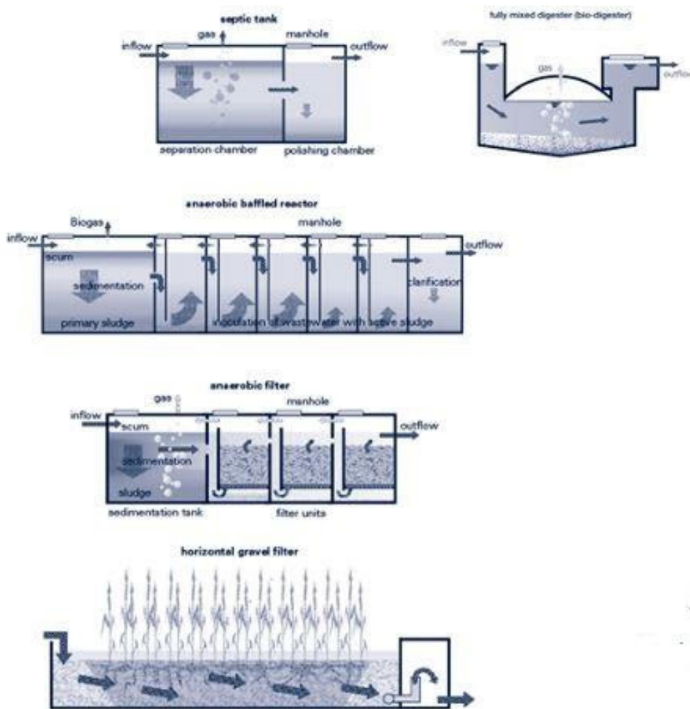
Figure 45: Treatment systems considered to be suitable for decentralised wastewater Treatment Systems 101
